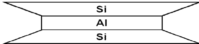
Fig. 4-10: Montmorillonite symbol
