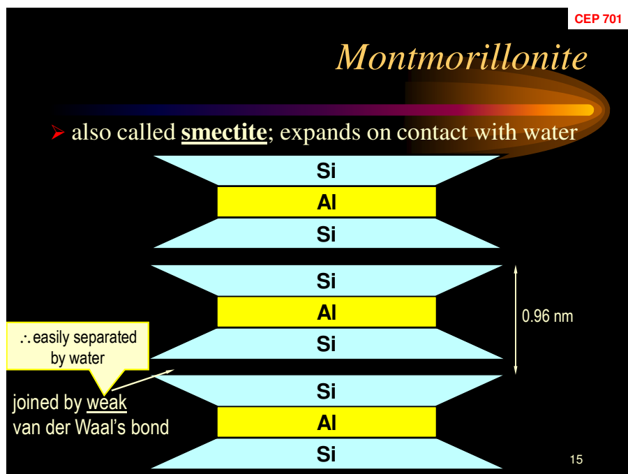
Fig. 4-11: Montmorillonite particles
