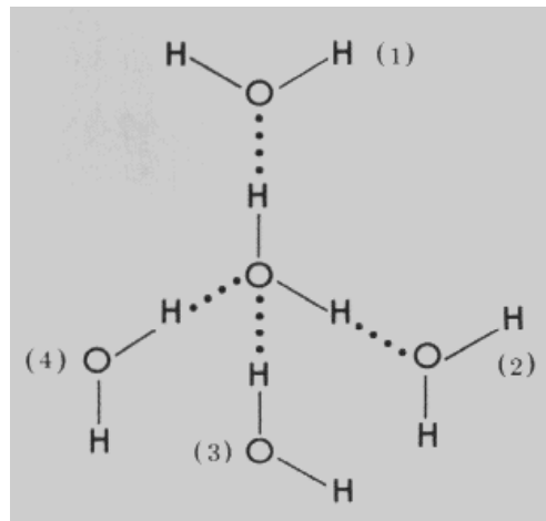
Fig. 4-3: Covalent bonding
