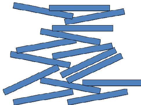
Fig. 4-16: Dispersed structure
